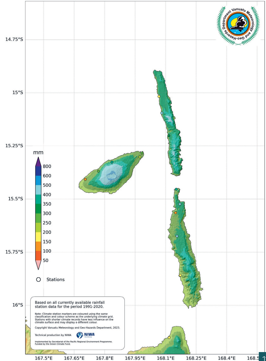
Penama: Mean November Rainfall
