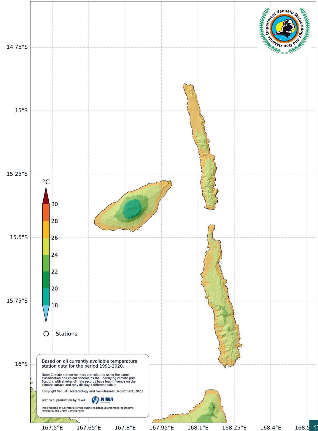
Penama: Mean May Temperature
