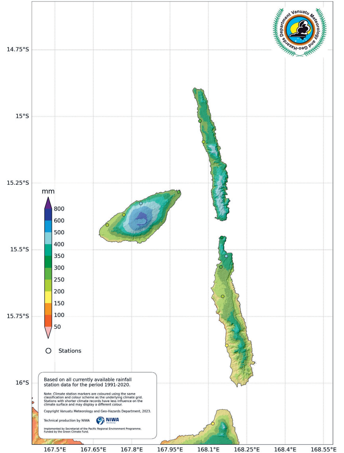
Penama: Mean May Rainfall
