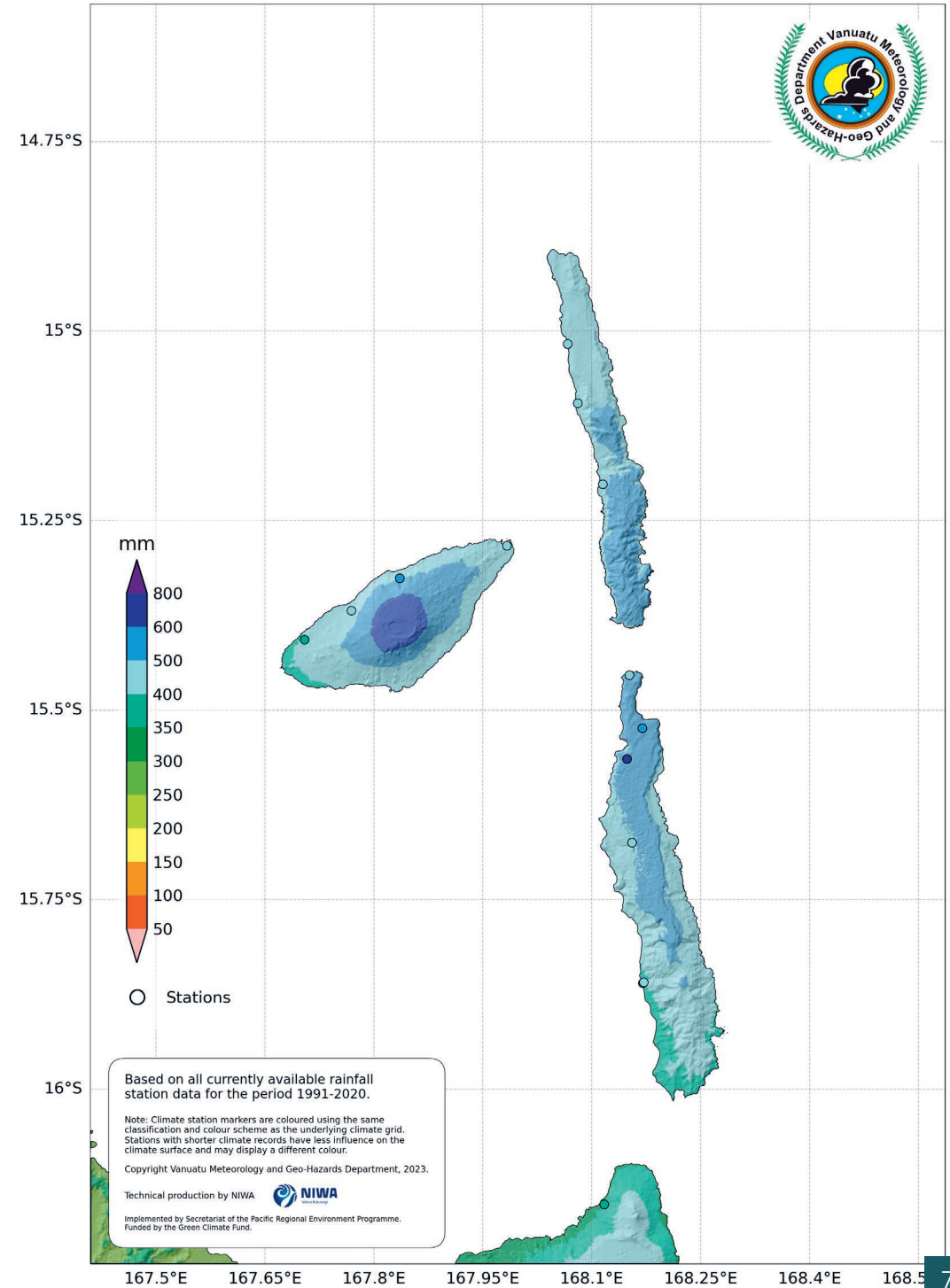
Penama: Mean March Rainfall
