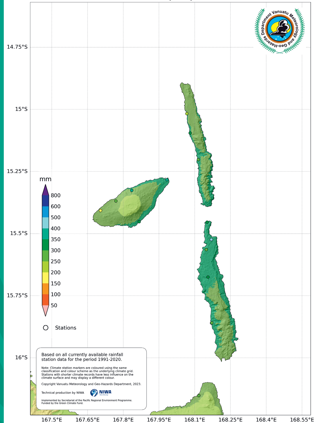
Penama: Mean January Rainfall
