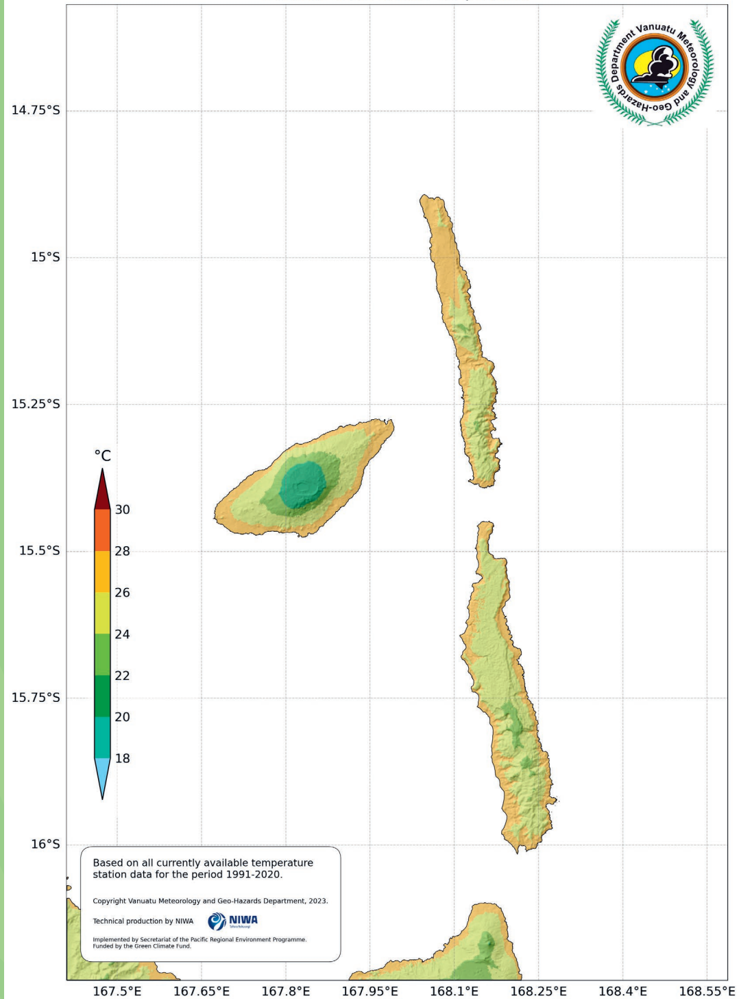
Penama: Mean Annual Temperature
