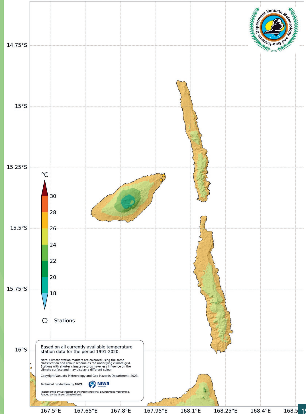
Penama: Mean January Temperature
