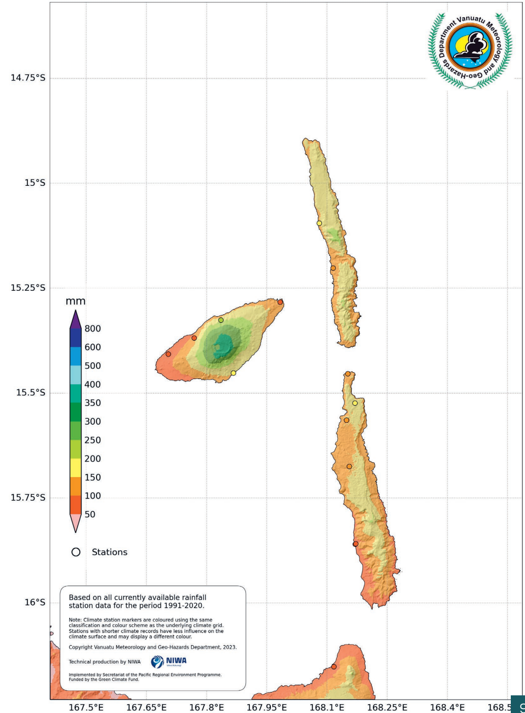
Penama: Mean July Rainfall
