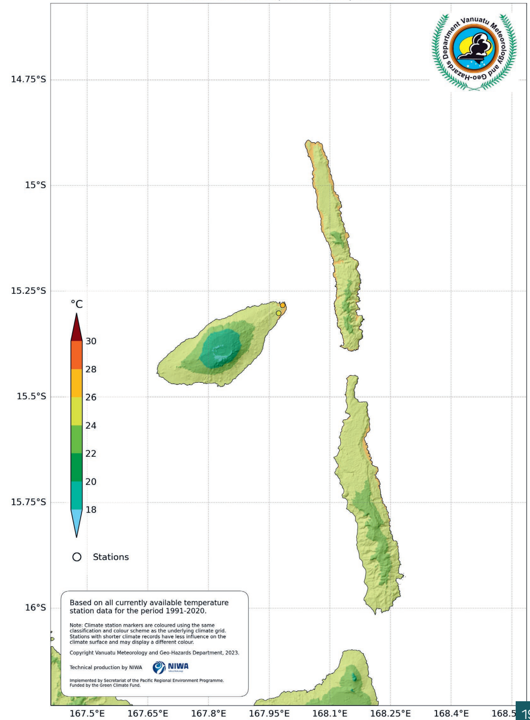
Penama: Mean September Temperature
