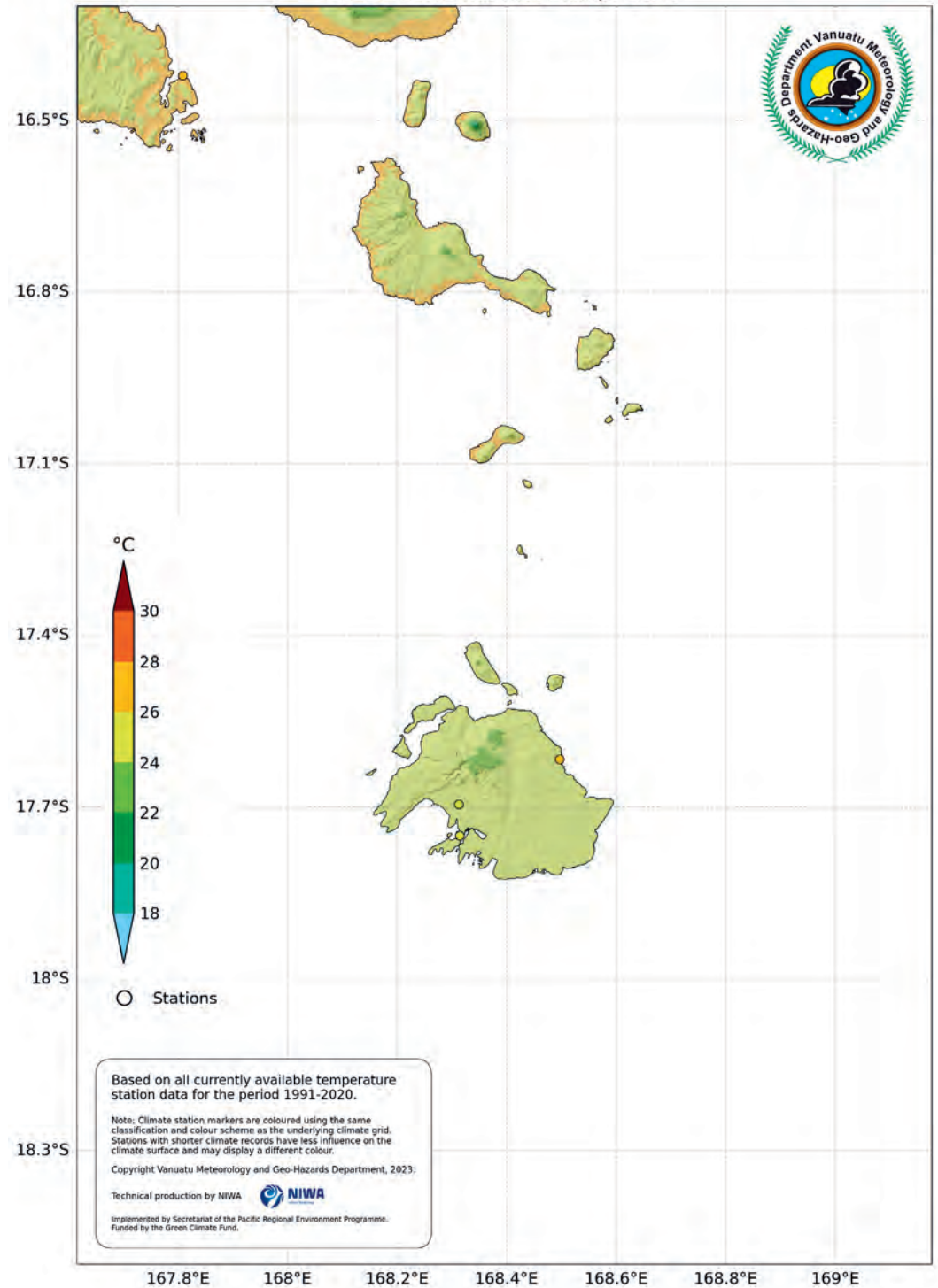
Shefa: Mean November Temperature
