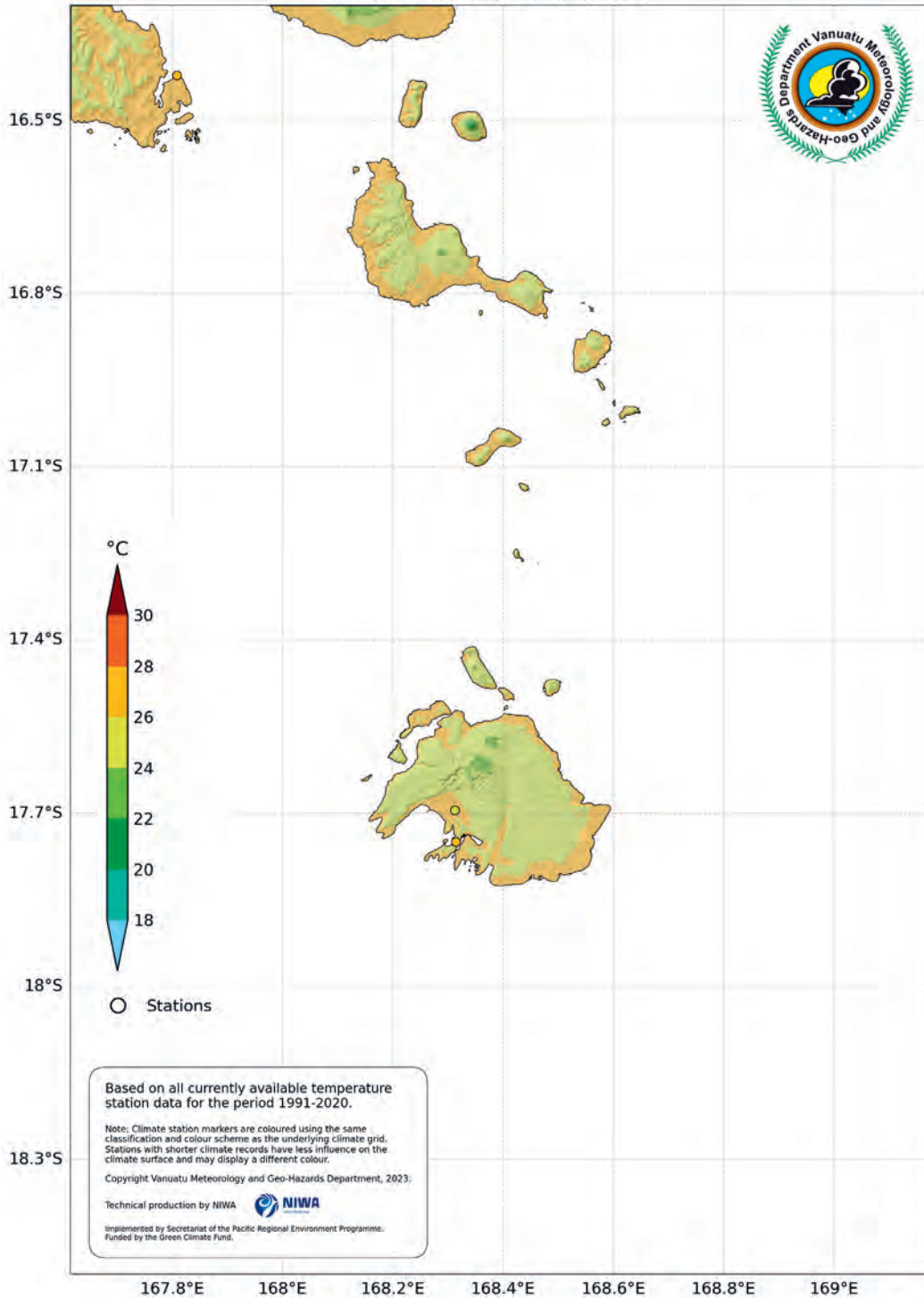
Shefa: Mean April Temperature
