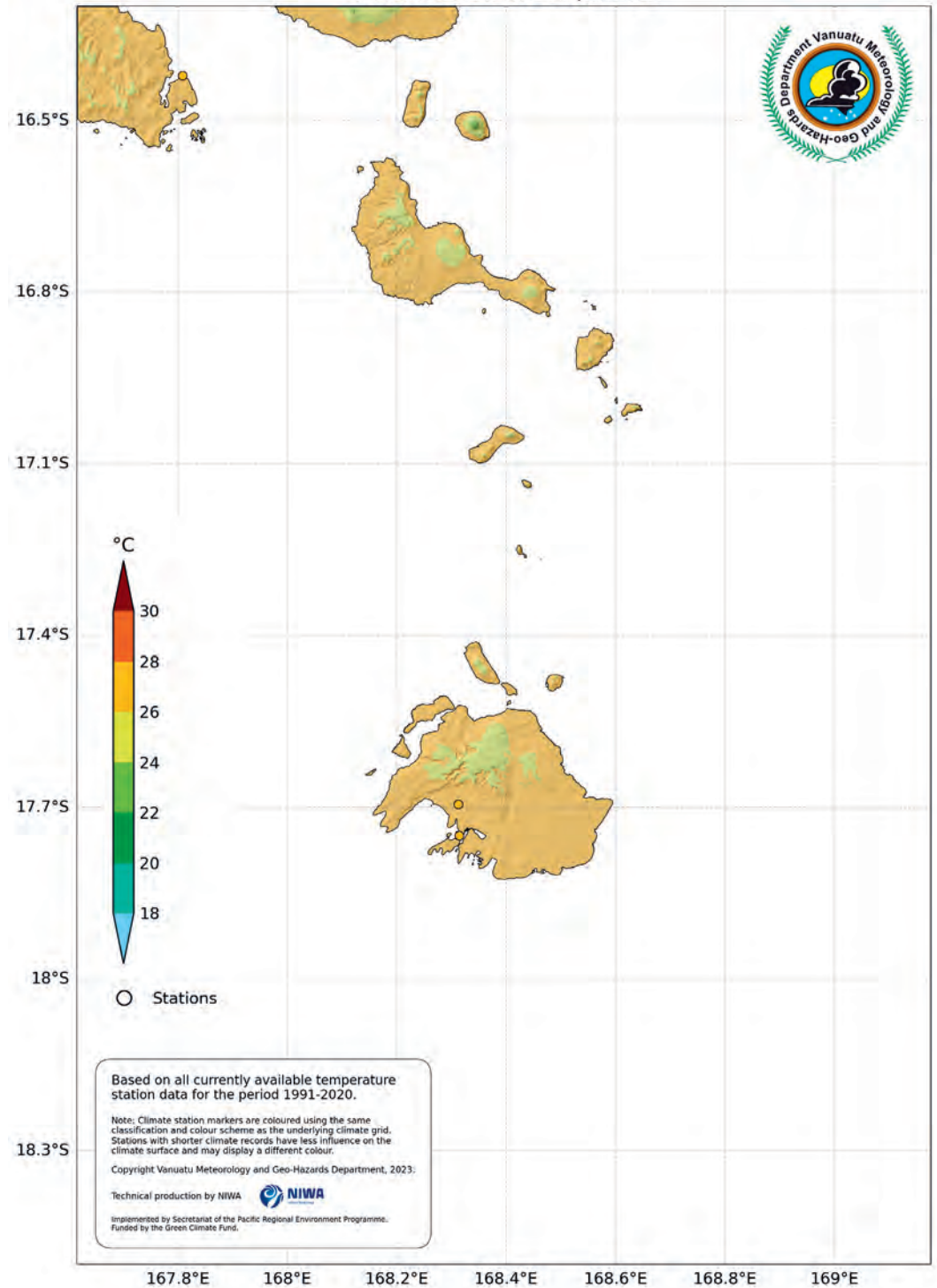
Shefa: Mean March Temperature
