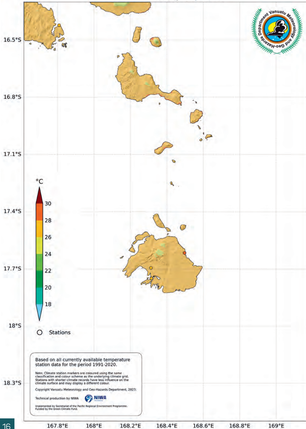
Shefa: Mean February Temperature
